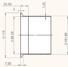
Tube – ferrule configuration
