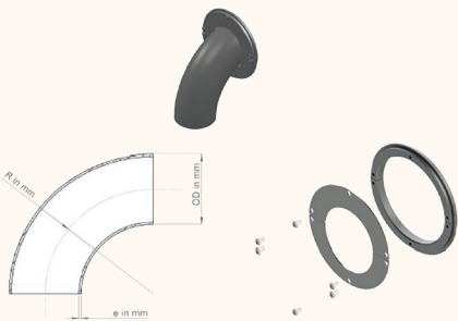
Tube – elbow configuration
