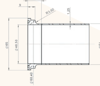
Tube – connector configuration
