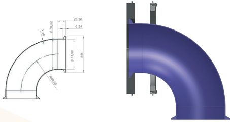
Ferrule – elbow – ferrule configuration (large diameter)
