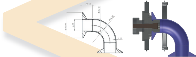
Ferrule – elbow – ferrule configuration (small diameter)
