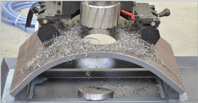
Base with permanent magnets can be adapted to a workpiece curvature
